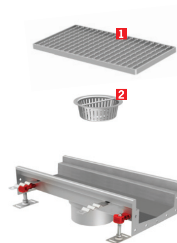
ACO modular box channel
